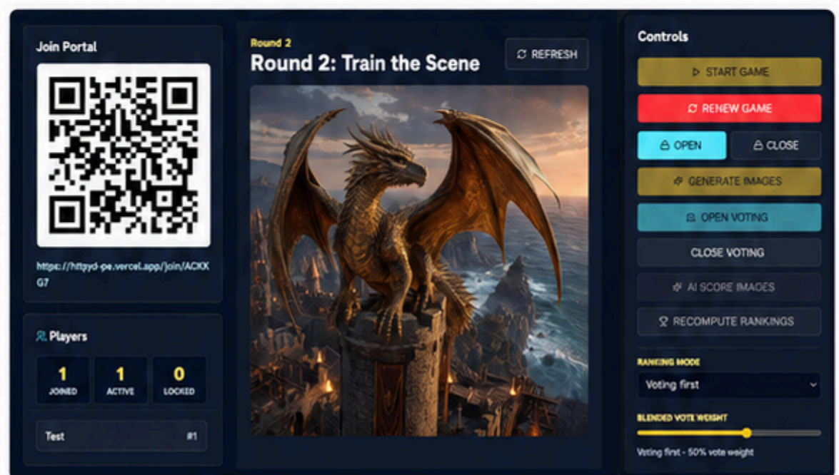
Figure 2. Host Round Screen (Example: Round 2)
